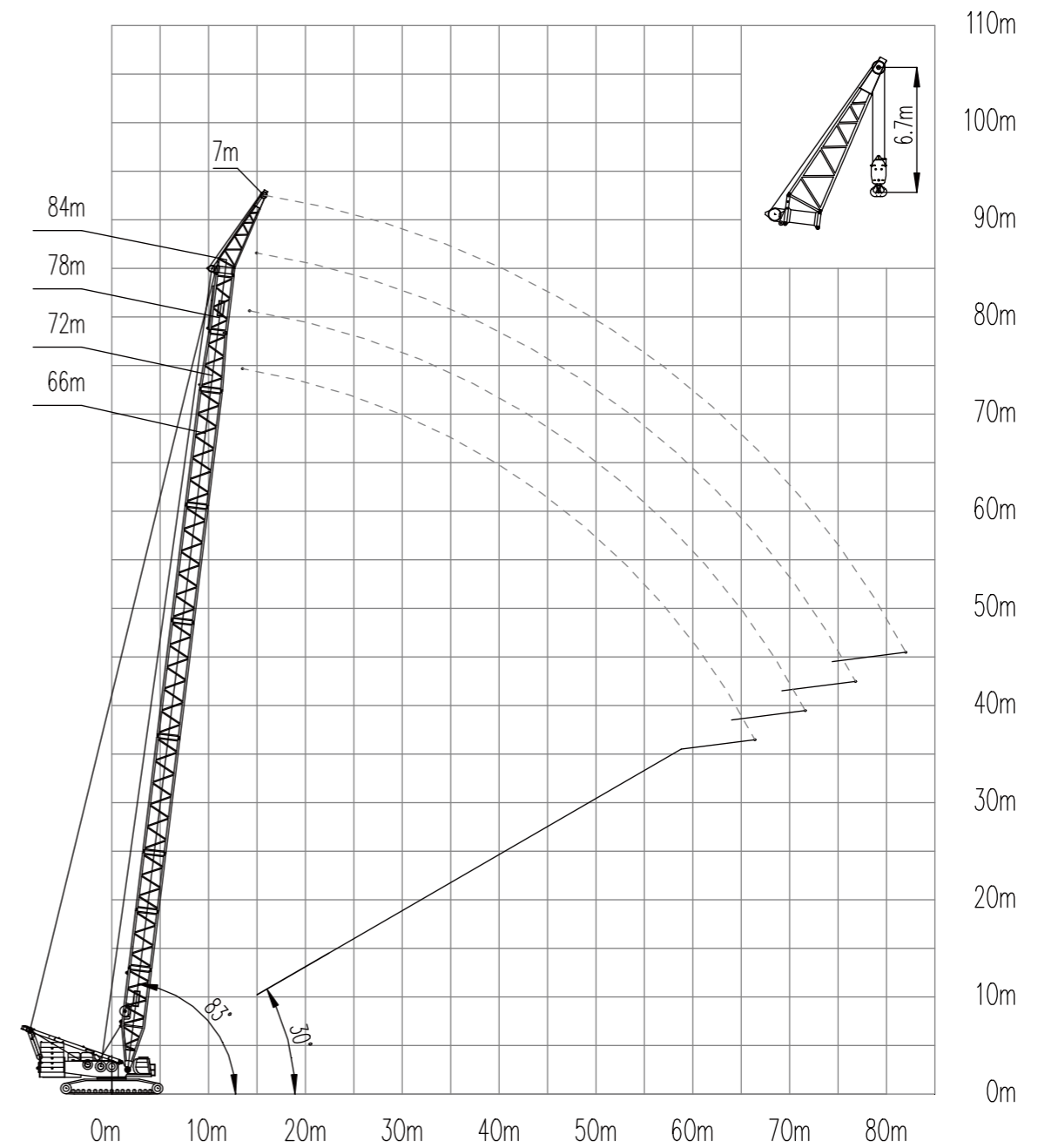
4. Standard goose head jib working condition (HJ)
